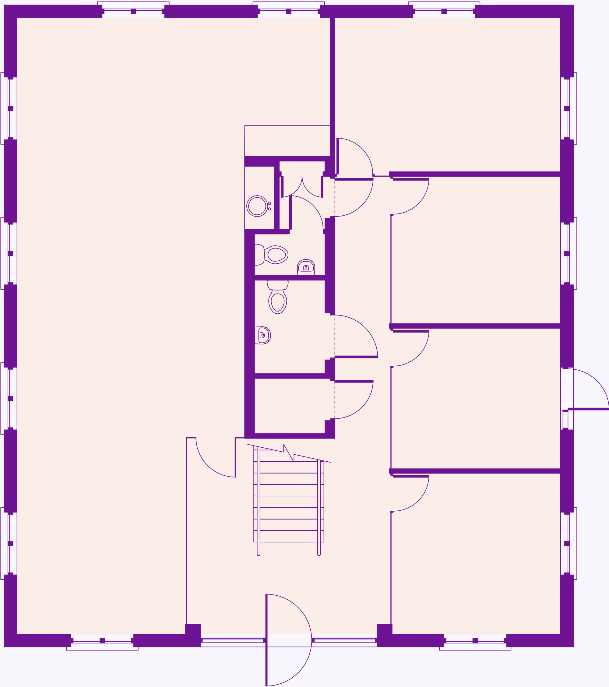
Ground floor
