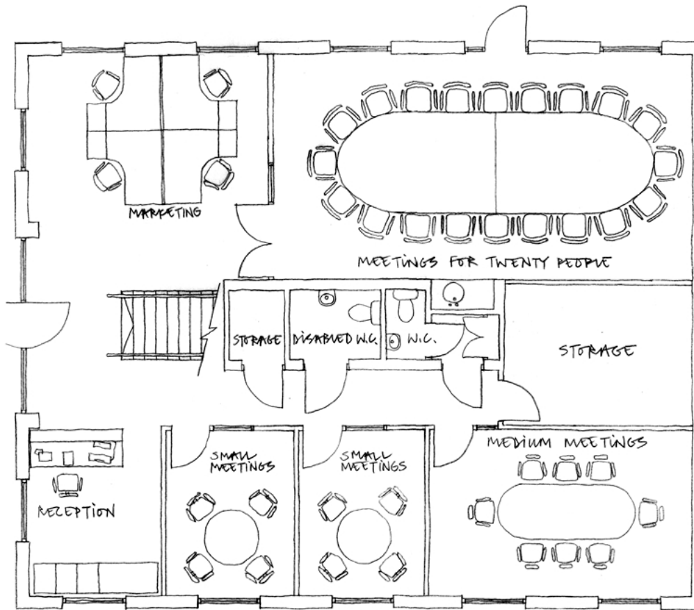
Unit One Ground Floor
