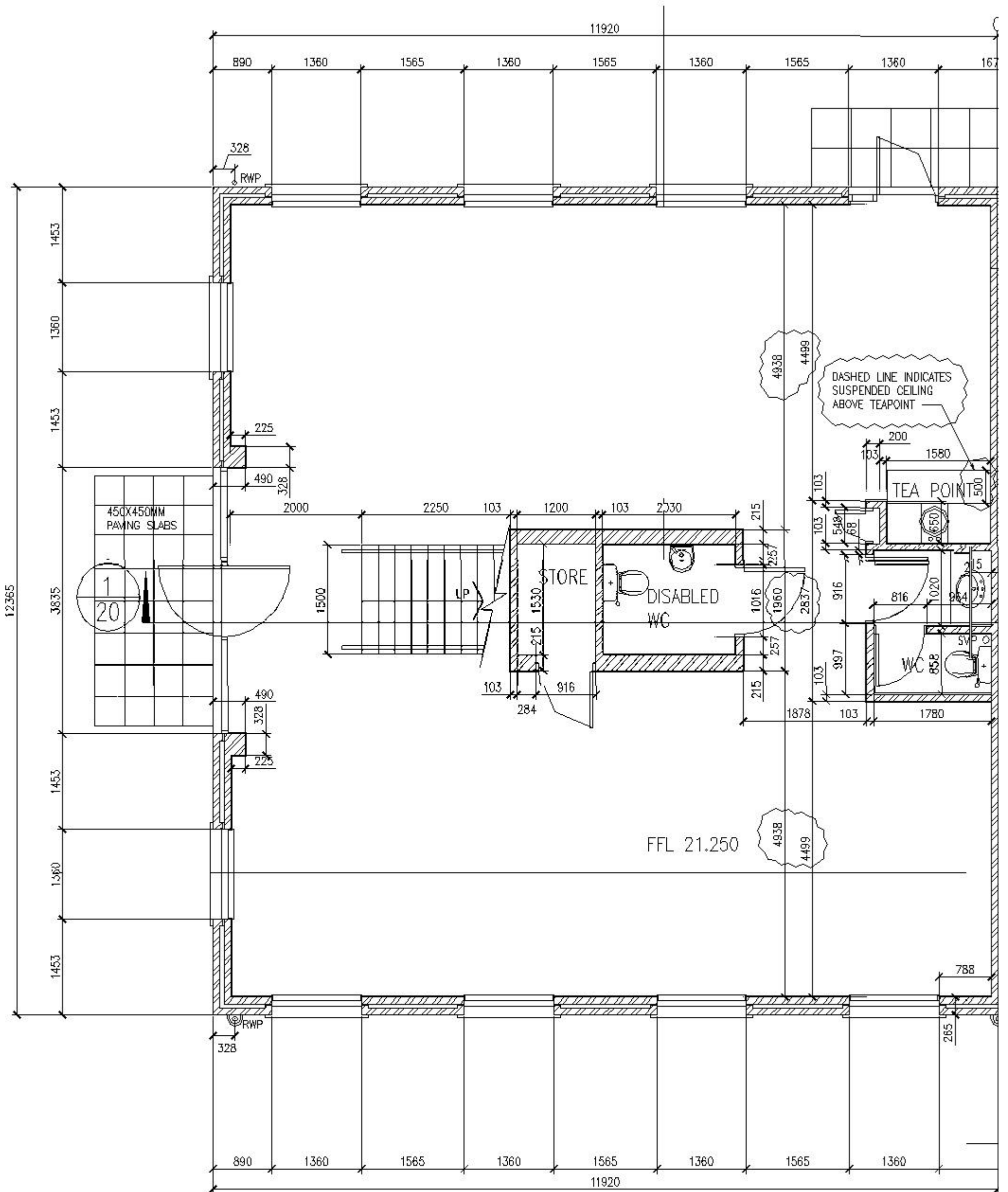
UNIT B GROUND FLOOR PLAN Scale 1:50
