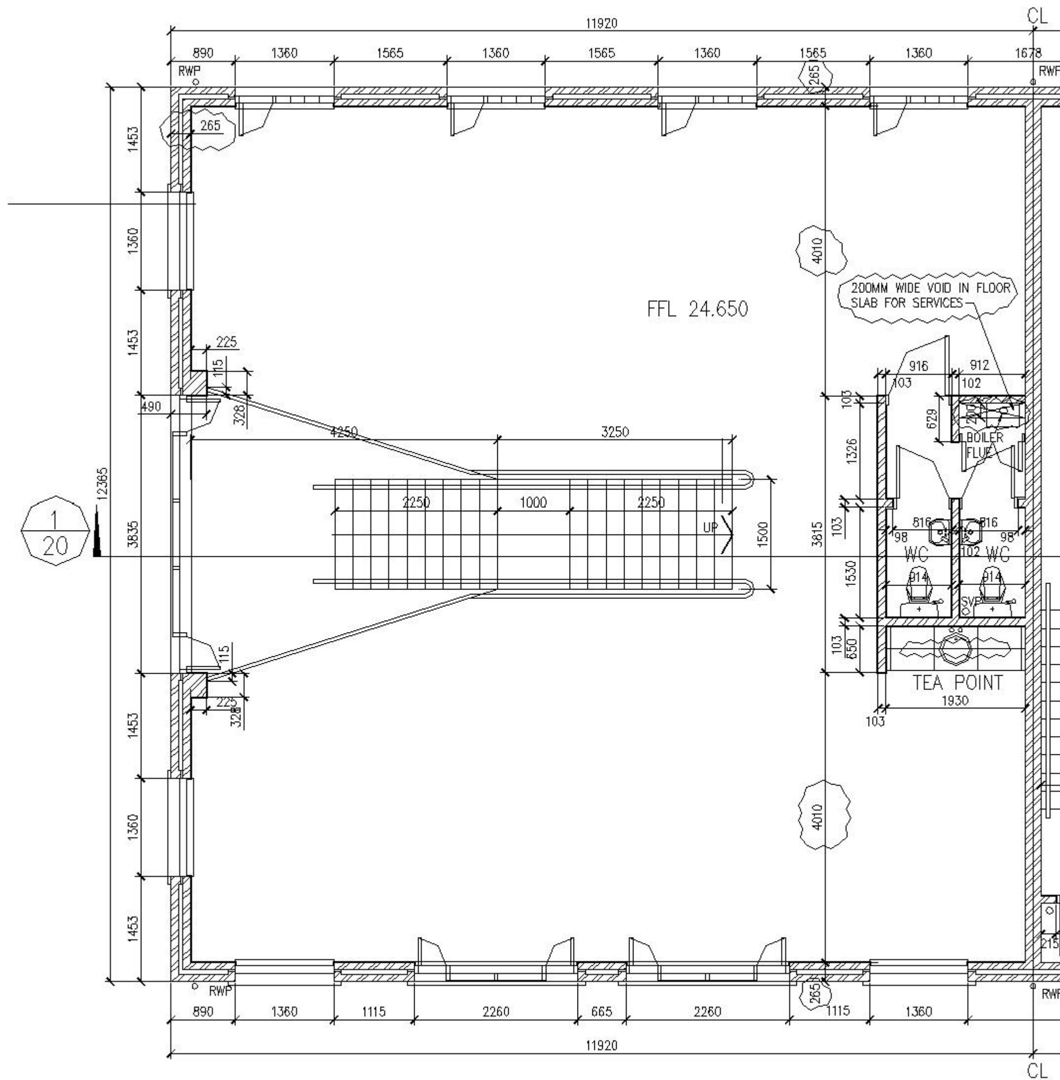
UNIT B FIRST FLOOR PLAN Scale 1:50
