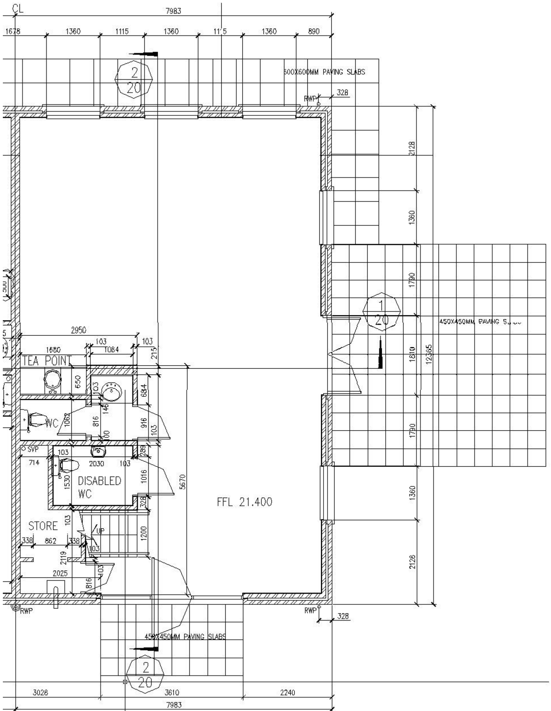
UNIT A GROUND FLOOR PLAN Scale
