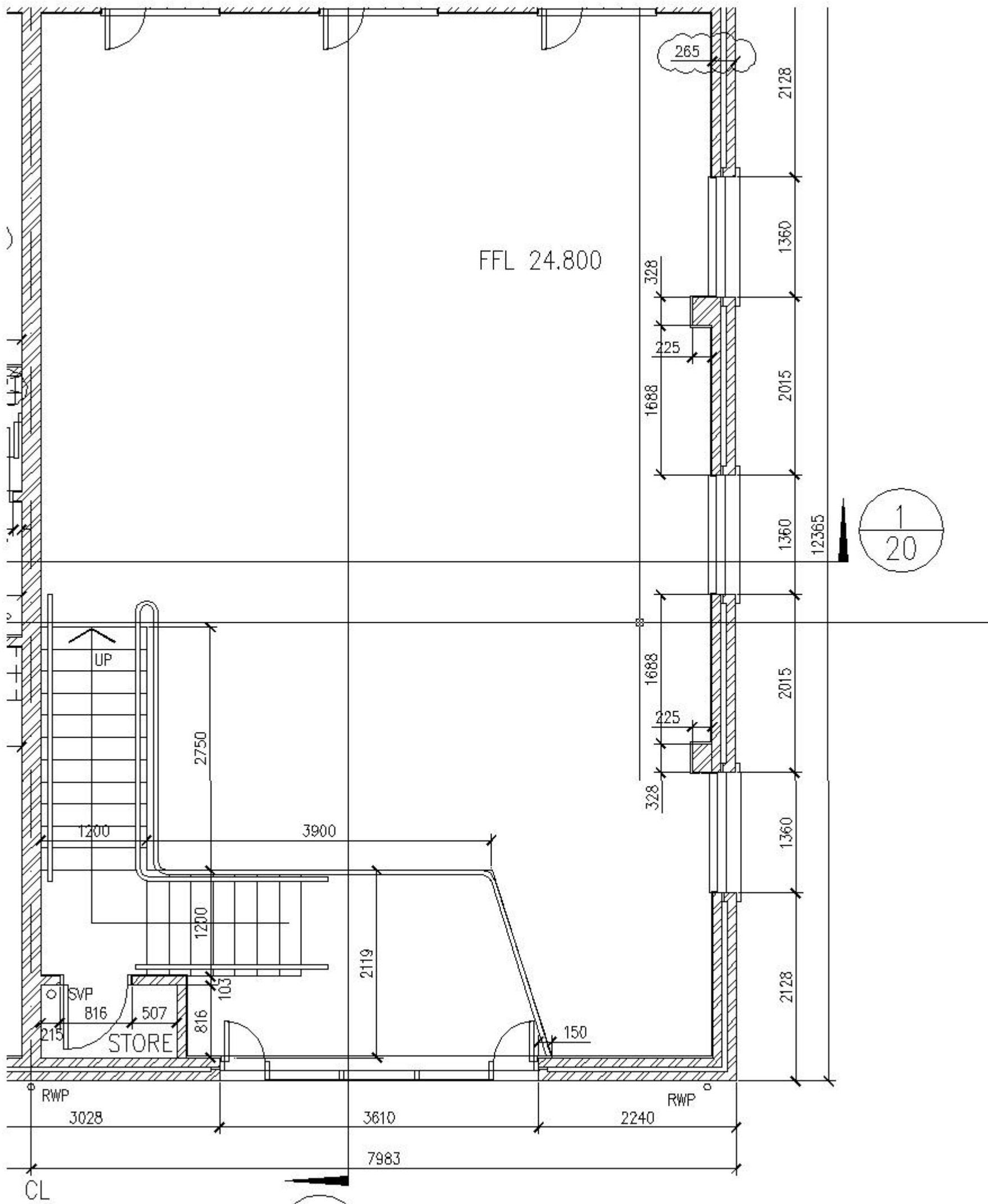
UNIT A FIRST FLOOR PLAN Scale 1:50
