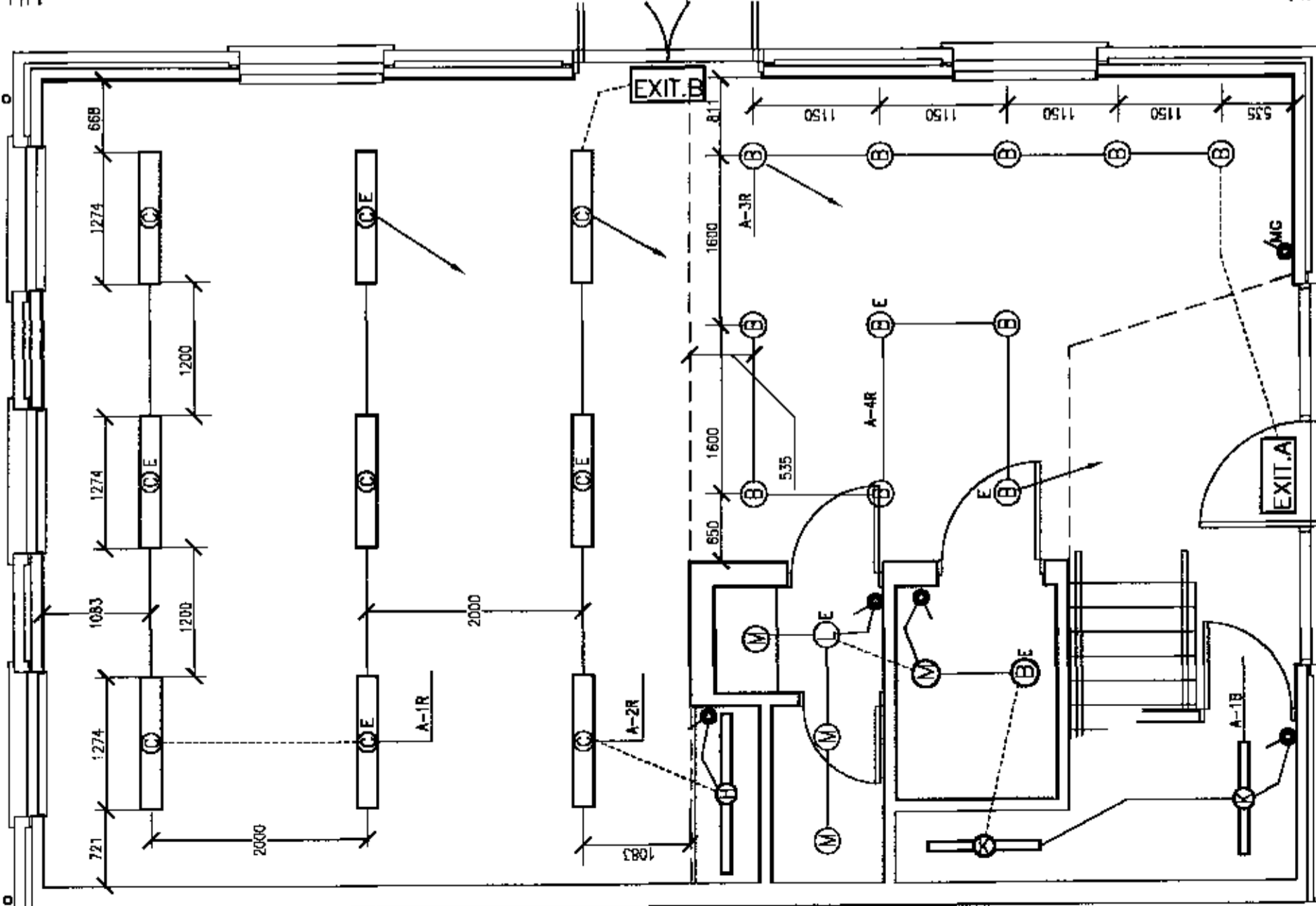
UNIT A - GROUND FLOOR PLAN
