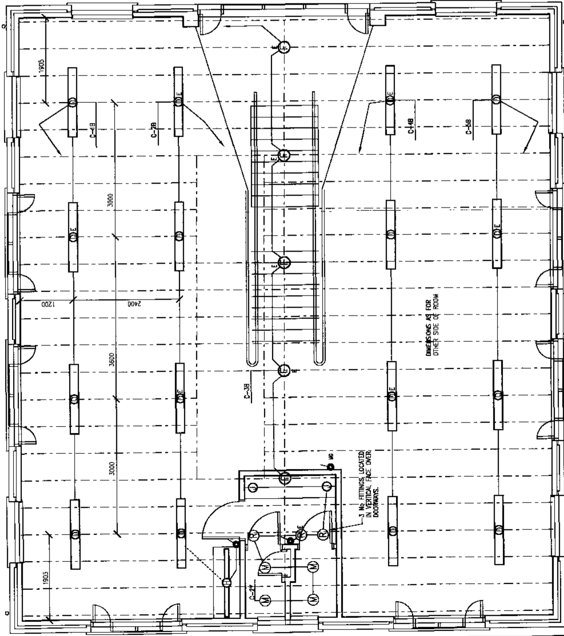
UNIT C - FIRST FLOOR PLAN
